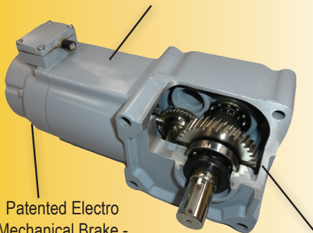
Hypoid/Helical Gears For Longevity
